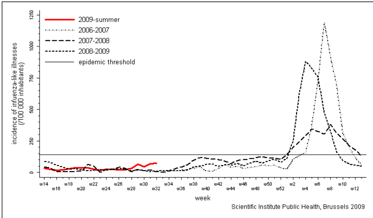
Figure 1: Evolution of ILI Incidence
